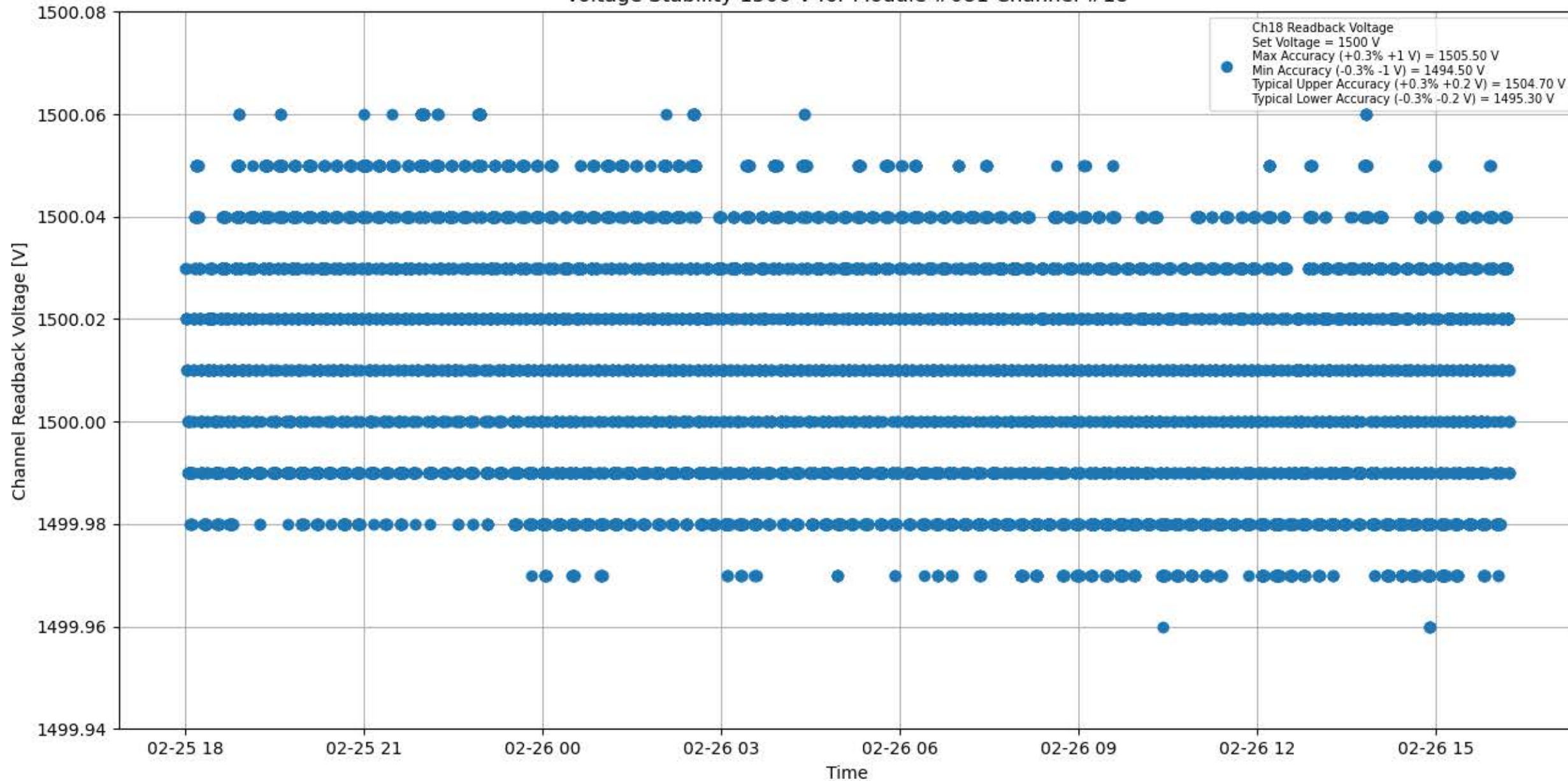
Voltage Stability 1500 V for Module #081 Channel #18
