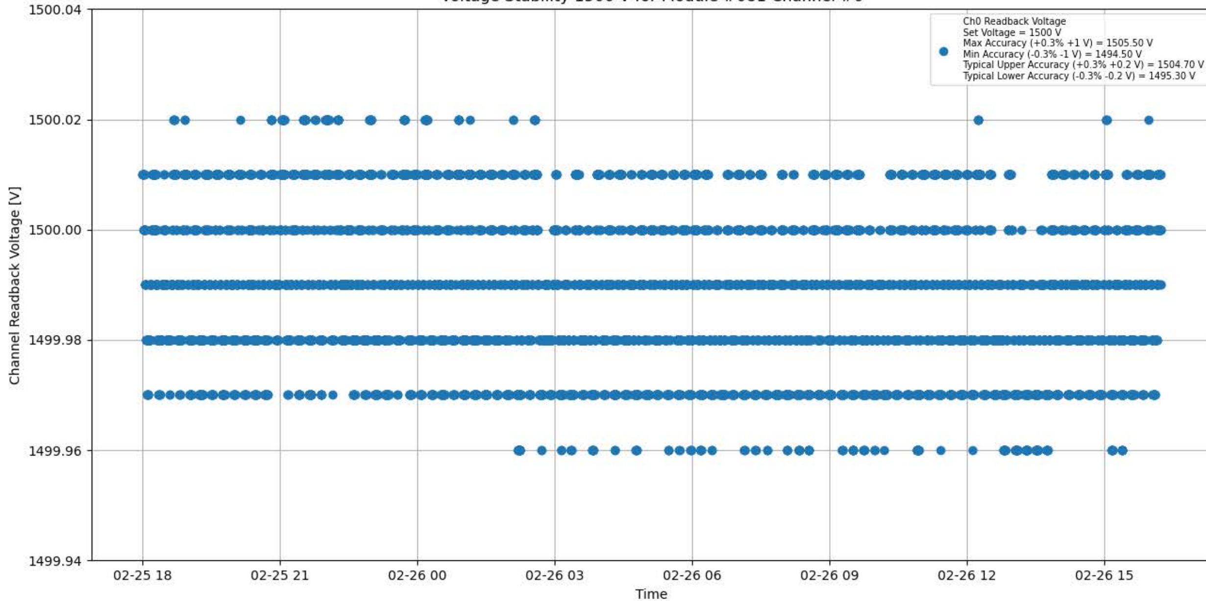
Voltage Stability 1500 V for Module #081 Channel #0
