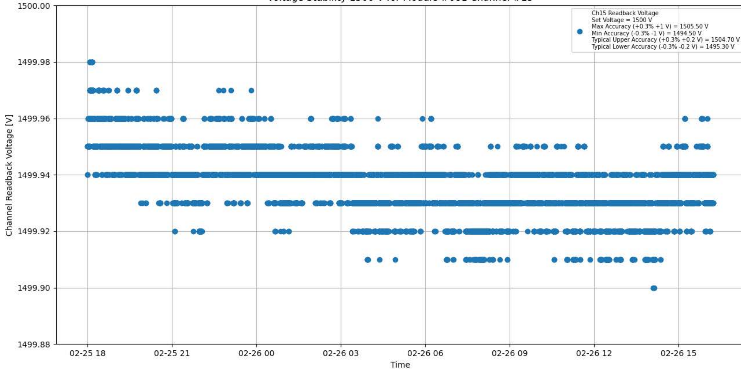
Voltage Stability 1500 V for Module #081 Channel #15
