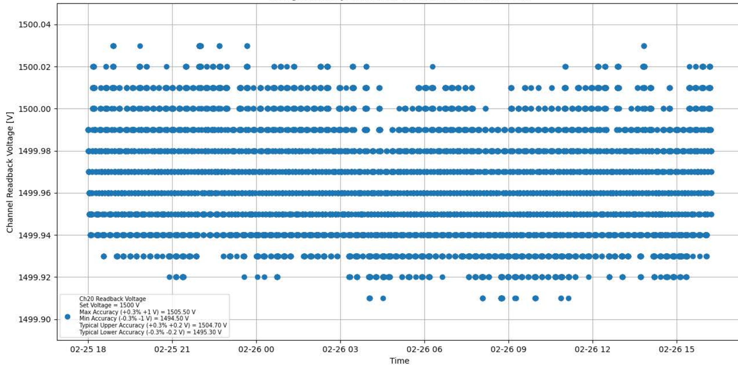
Voltage Stability 1500 V for Module #081 Channel #20
