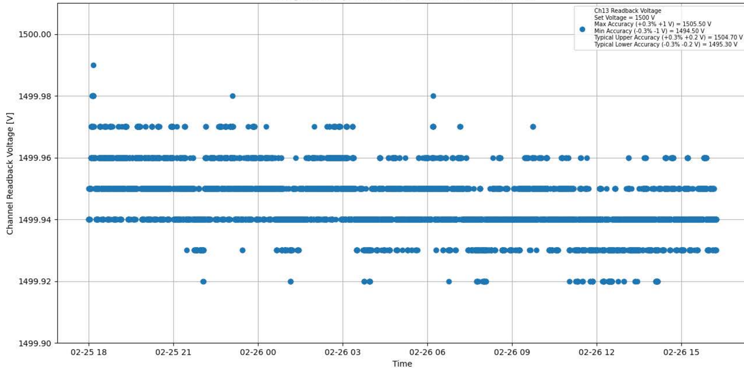
Voltage Stability 1500 V for Module #081 Channel #13
