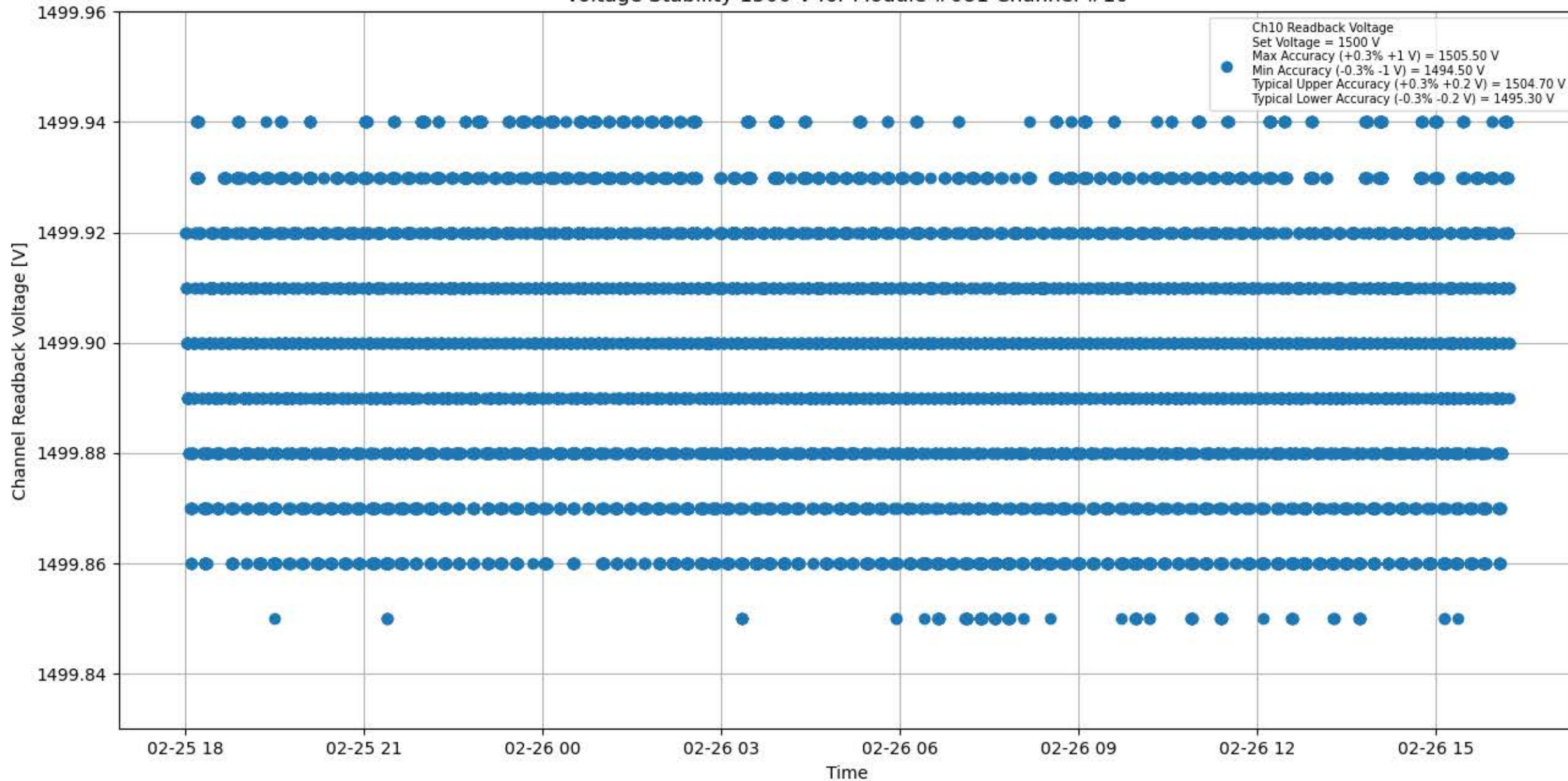
Voltage Stability 1500 V for Module #081 Channel #10
