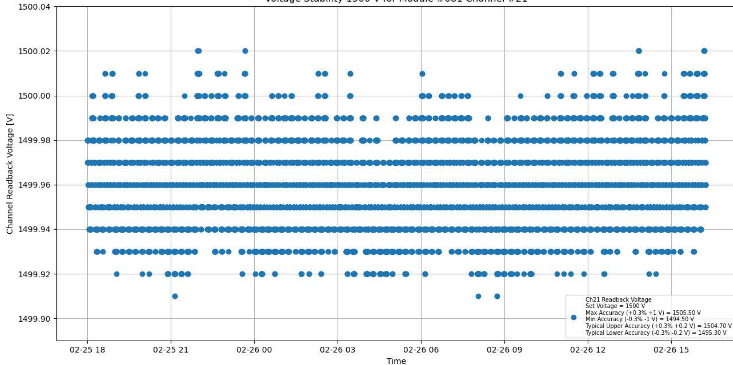
Voltage Stability 1500 V for Module #081 Channel #21
