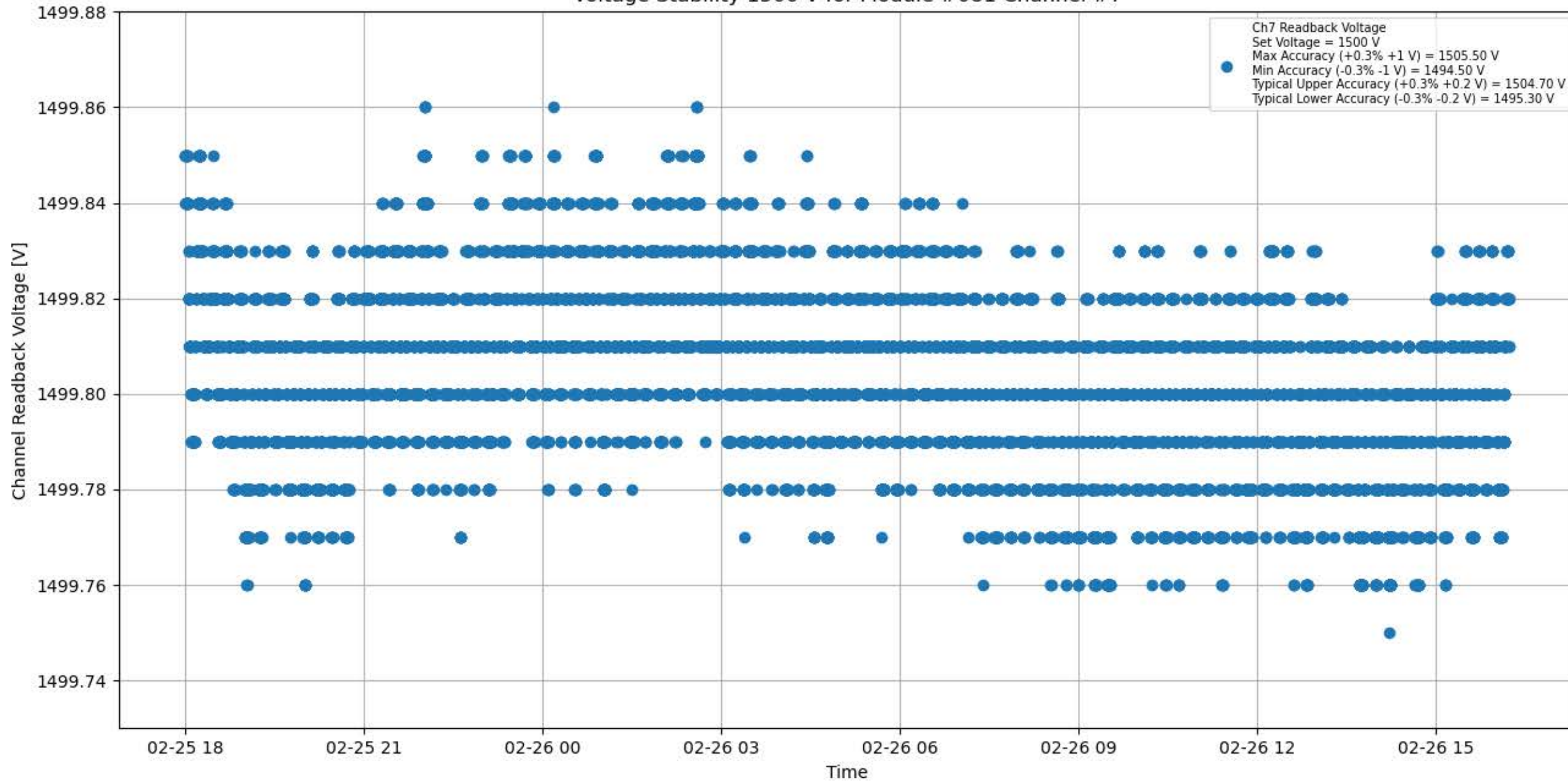
Voltage Stability 1500 V for Module #081 Channel #7
