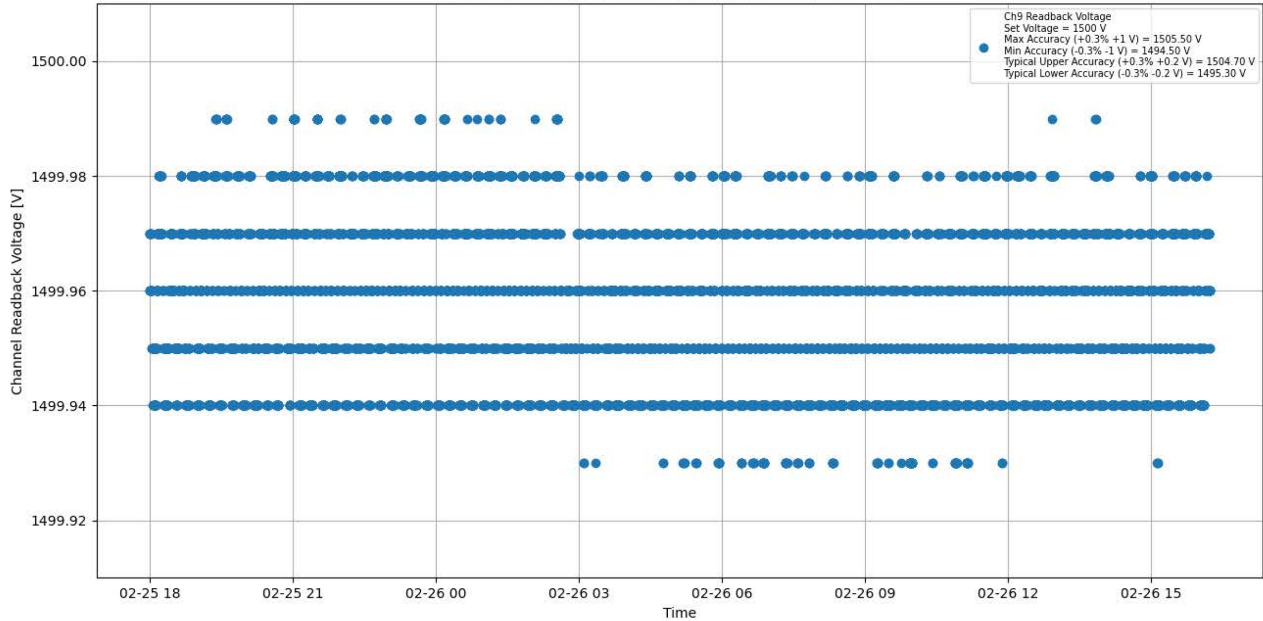
Voltage Stability 1500 V for Module #081 Channel #9
