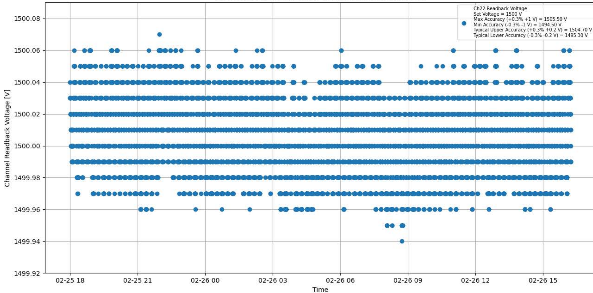
Voltage Stability 1500 V for Module #081 Channel #22
