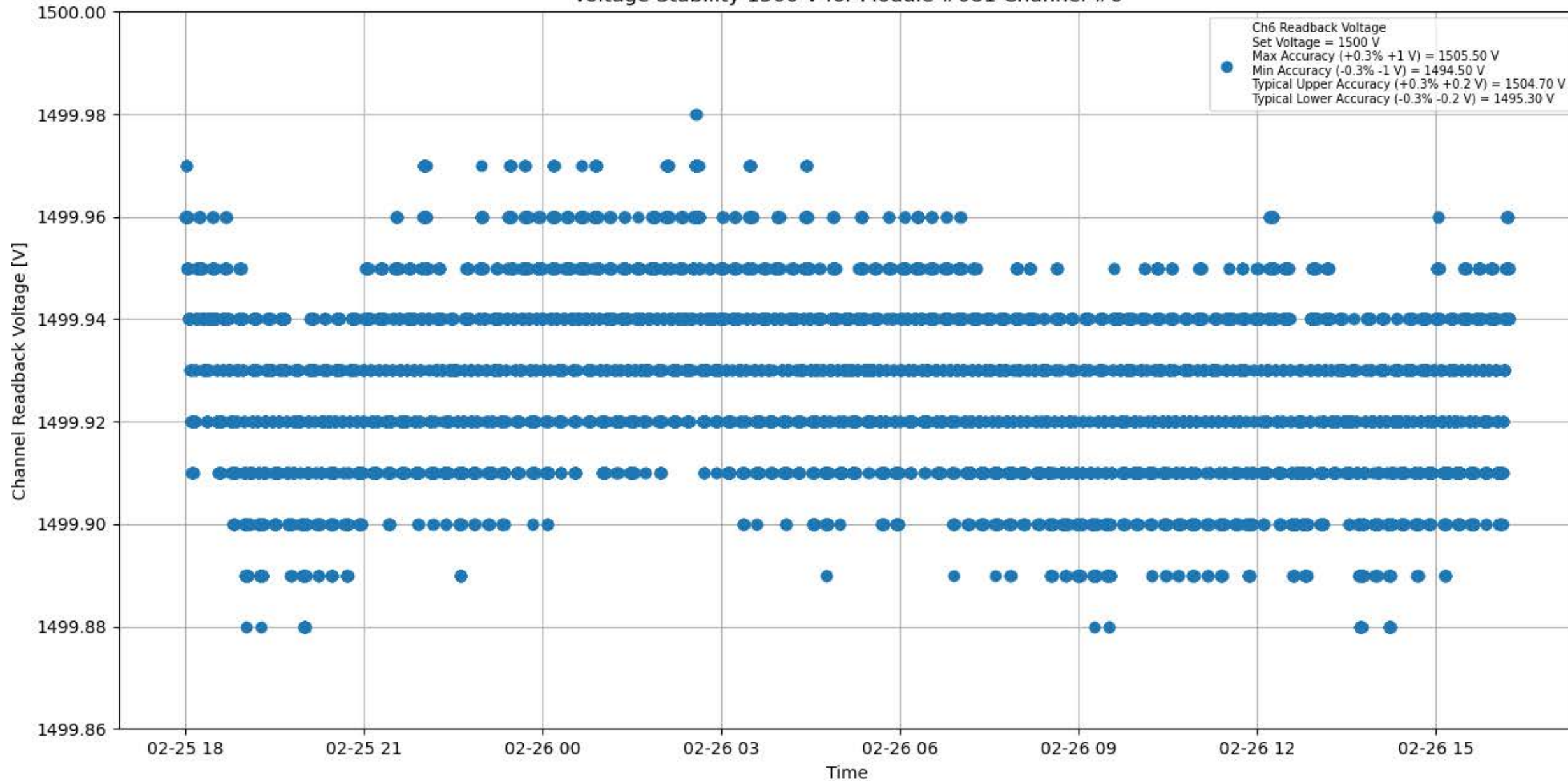
Voltage Stability 1500 V for Module #081 Channel #6
