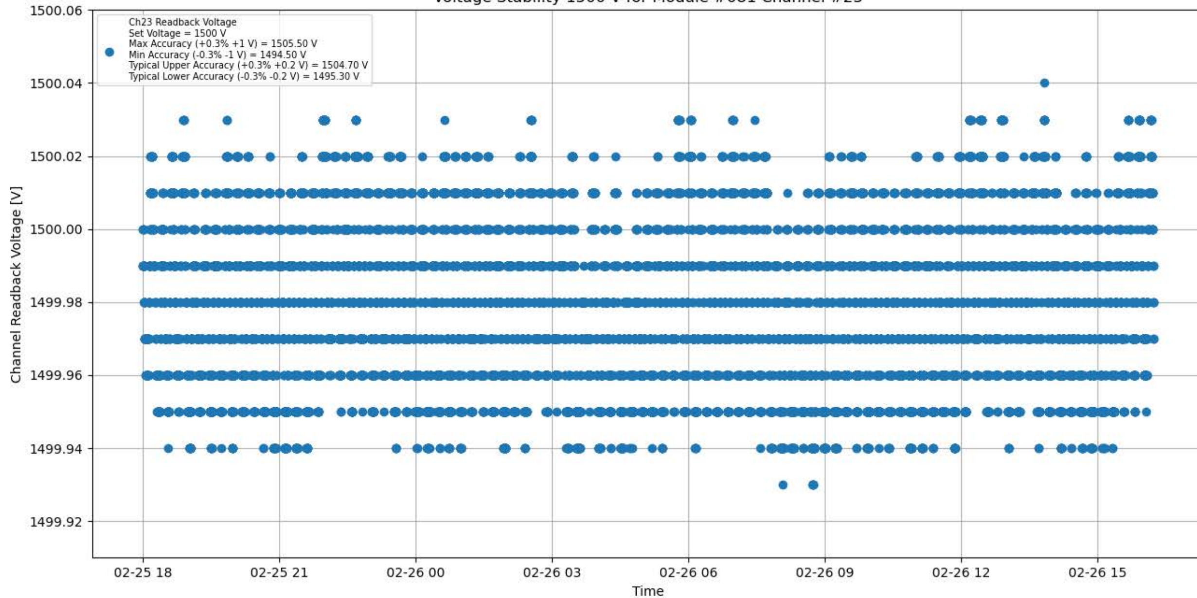
Voltage Stability 1500 V for Module #081 Channel #23
