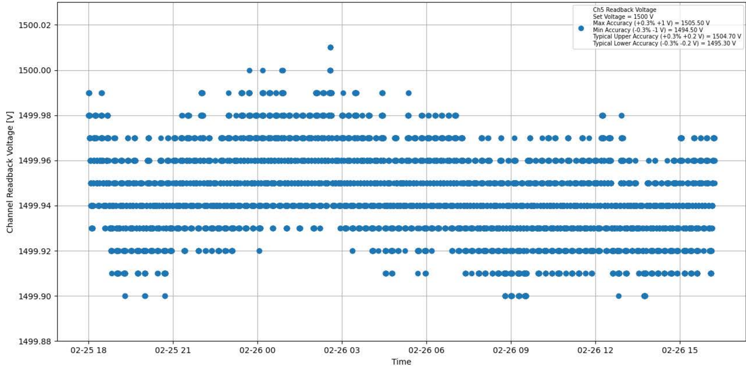
Voltage Stability 1500 V for Module #081 Channel #5
