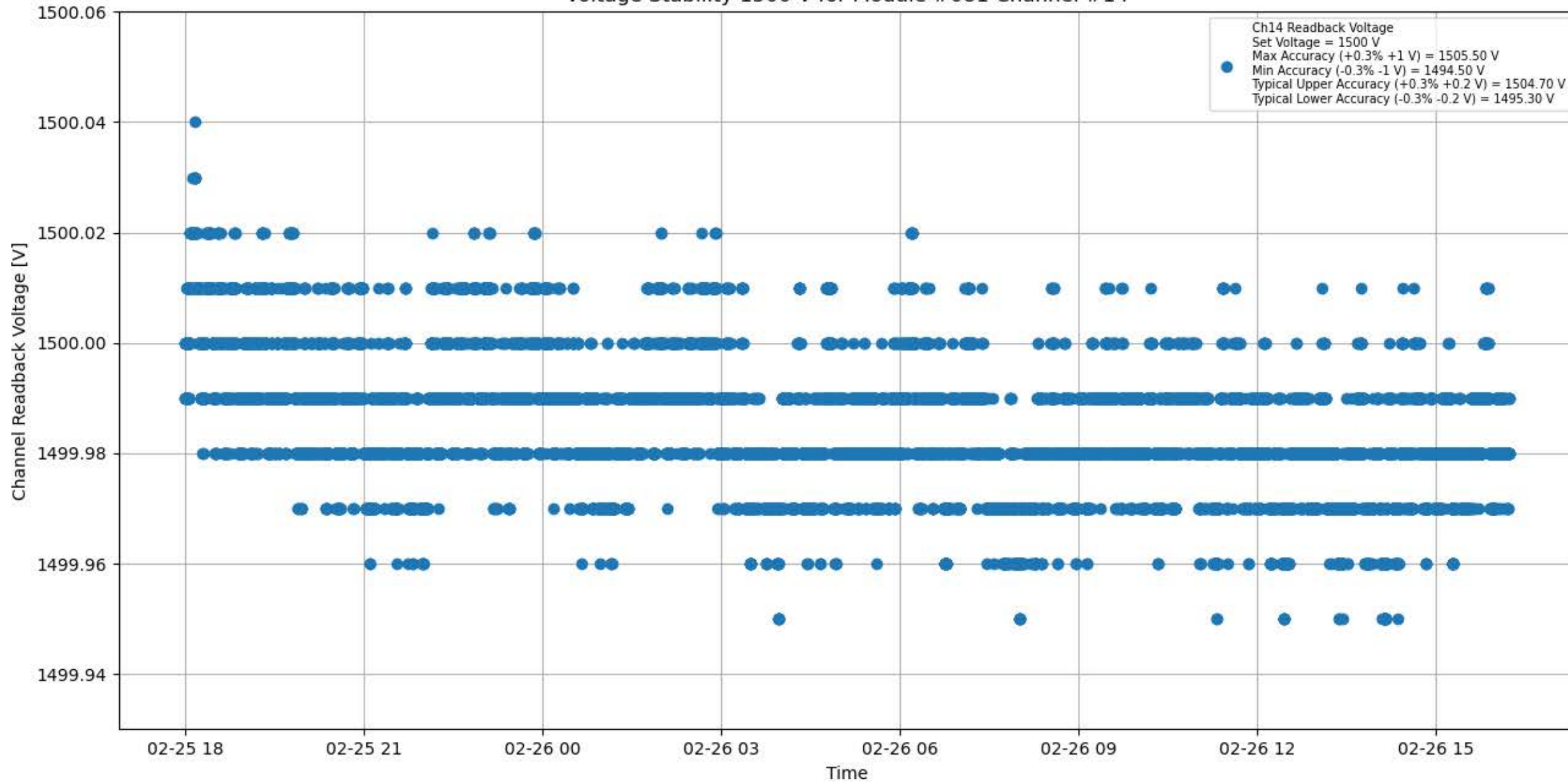
Voltage Stability 1500 V for Module #081 Channel #14
