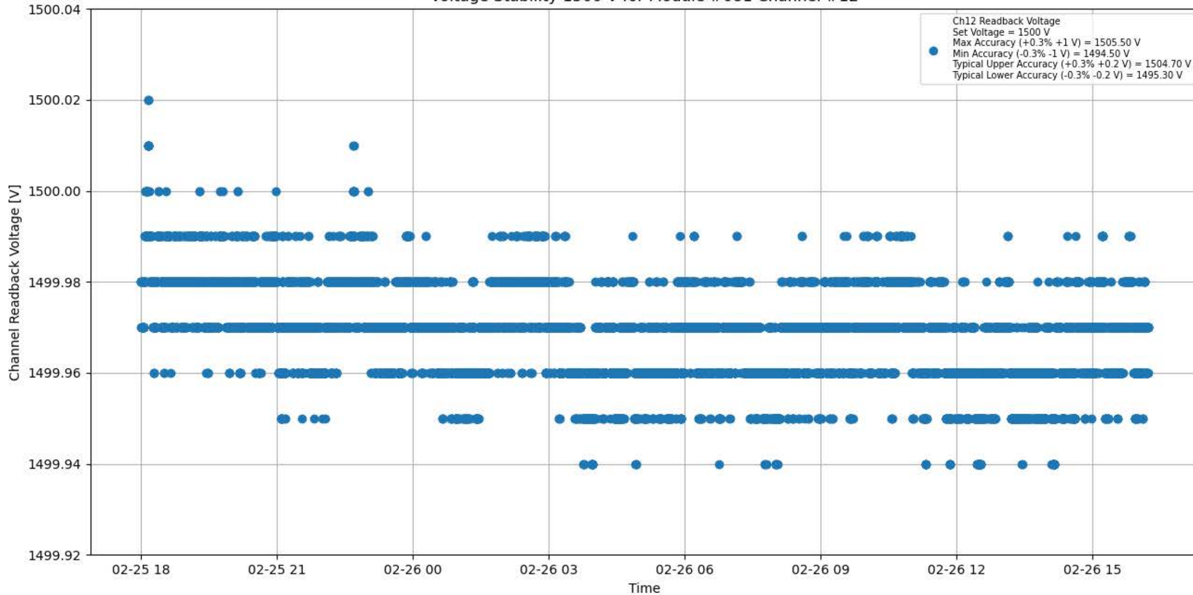
Voltage Stability 1500 V for Module #081 Channel #12
