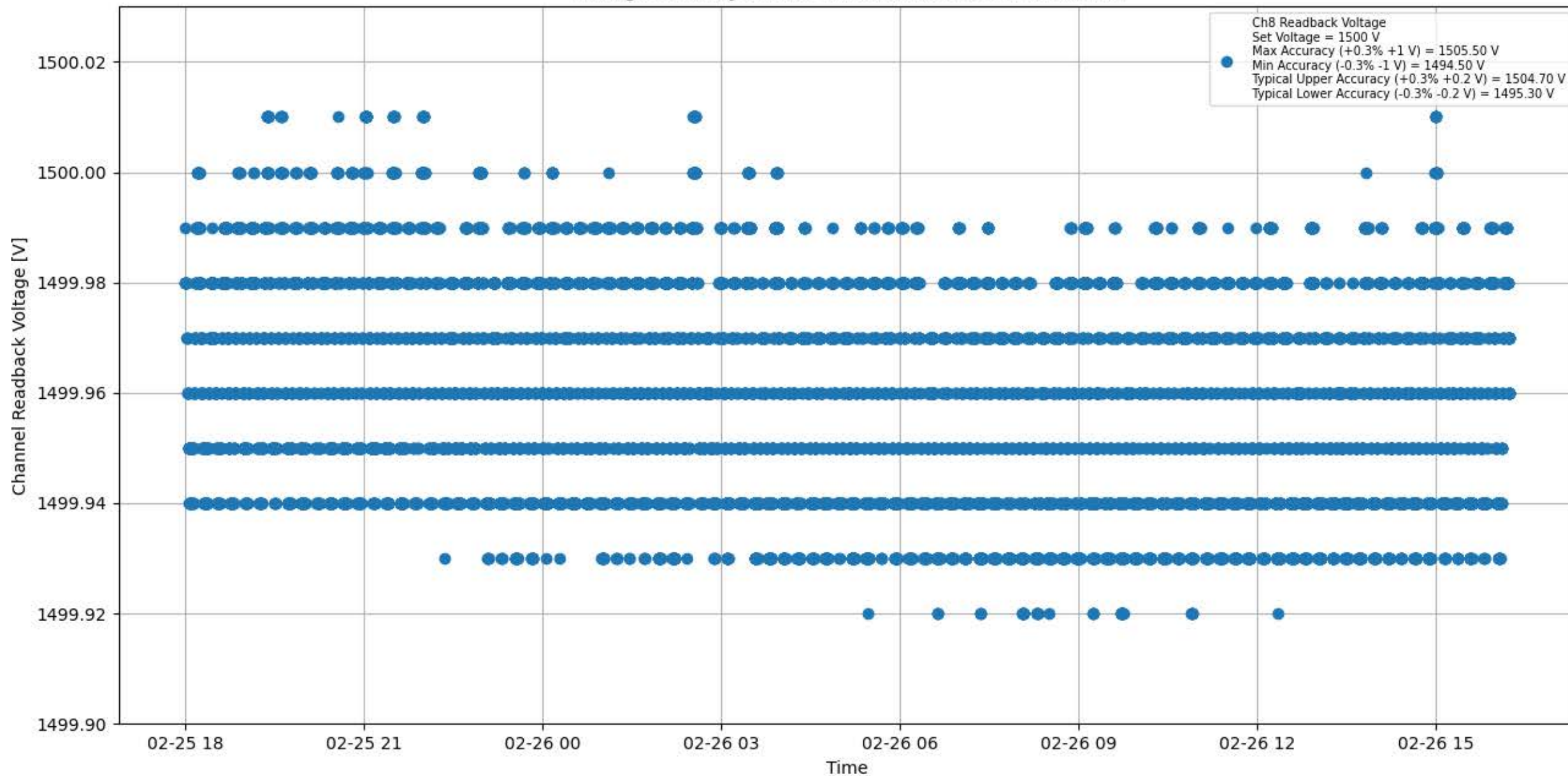
Voltage Stability 1500 V for Module #081 Channel #8
