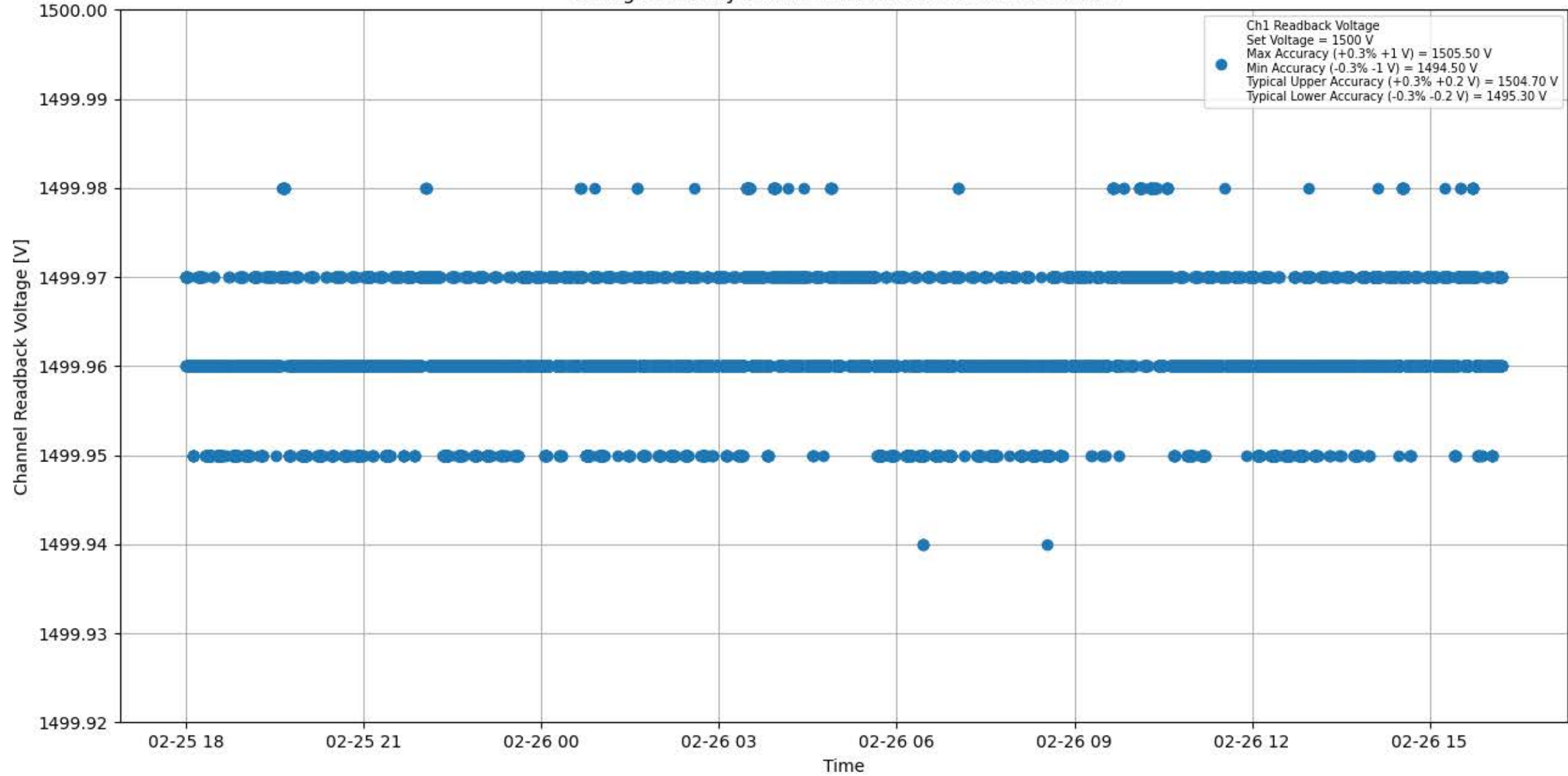
Voltage Stability 1500 V for Module #081 Channel #1
