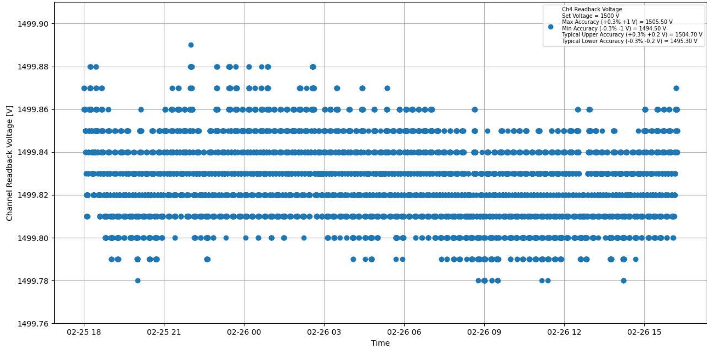
Voltage Stability 1500 V for Module #081 Channel #4
